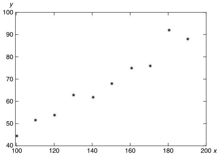
FIGURE 9.1 Scatter plot.
