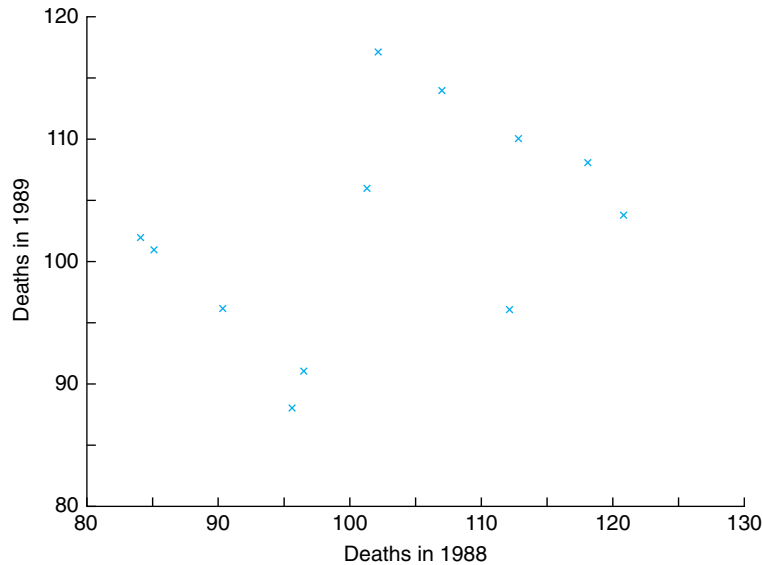
FIGURE 9.8 Scatter diagram of 1989 deaths versus 1988 deaths.
