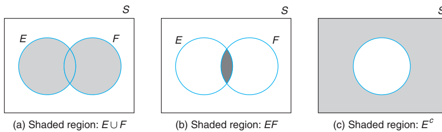
FIGURE 3.1 Venn diagrams.
